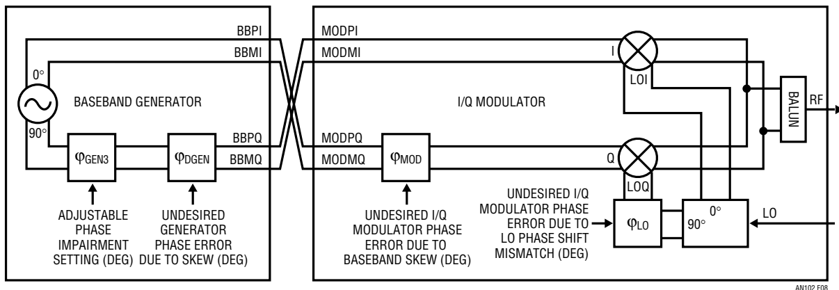
Figure 8. Measurement Setup for Configuration 3
