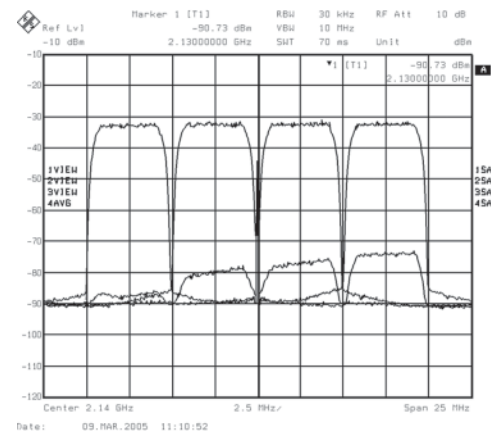
Figure 2. Measurement Compilation of Four One-Channel W-CDMA I/Q Modulator RF Output Spectra Selected to be at -7.5MHz, -2.5MHz, 2.5MHz and 7.5MHz Offset Frequency from the 2.14GHz Carrier Using Baseband I/Q W-CDMA Channel Selection with Uncalibrated Image
