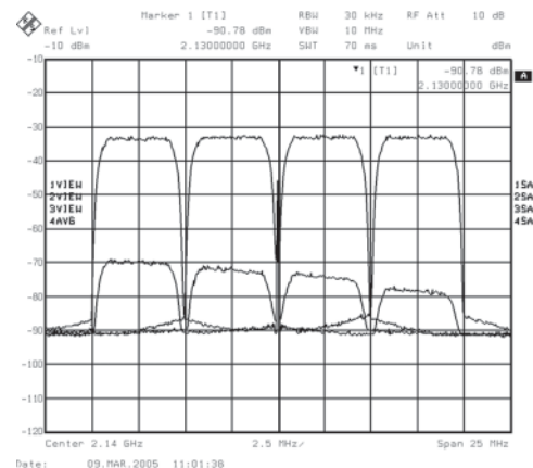
Figure 1. Measurement Compilation of Four One-Channel W-CDMA I/Q Modulator RF Output Spectra Selected to be at -7.5MHz, -2.5MHz, 2.5MHz and 7.5MHz Offset Frequency from the 2.14GHz Carrier Using Baseband I/Q W-CDMA Channel Selection with Uncalibrated Image
