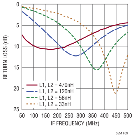
Figure 9. IF Output Return Loss Bandpass Matching with 4:1 Transformer
